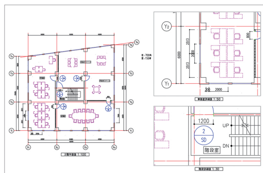
[異縮尺図面]
